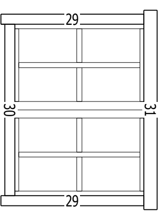
DOUBLE WINDOW 1380X1050
