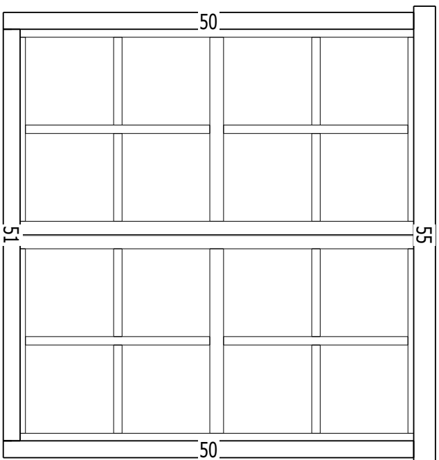
FIXED WINDOW 2000X1935
