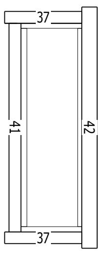
WINDOW 1450X450
