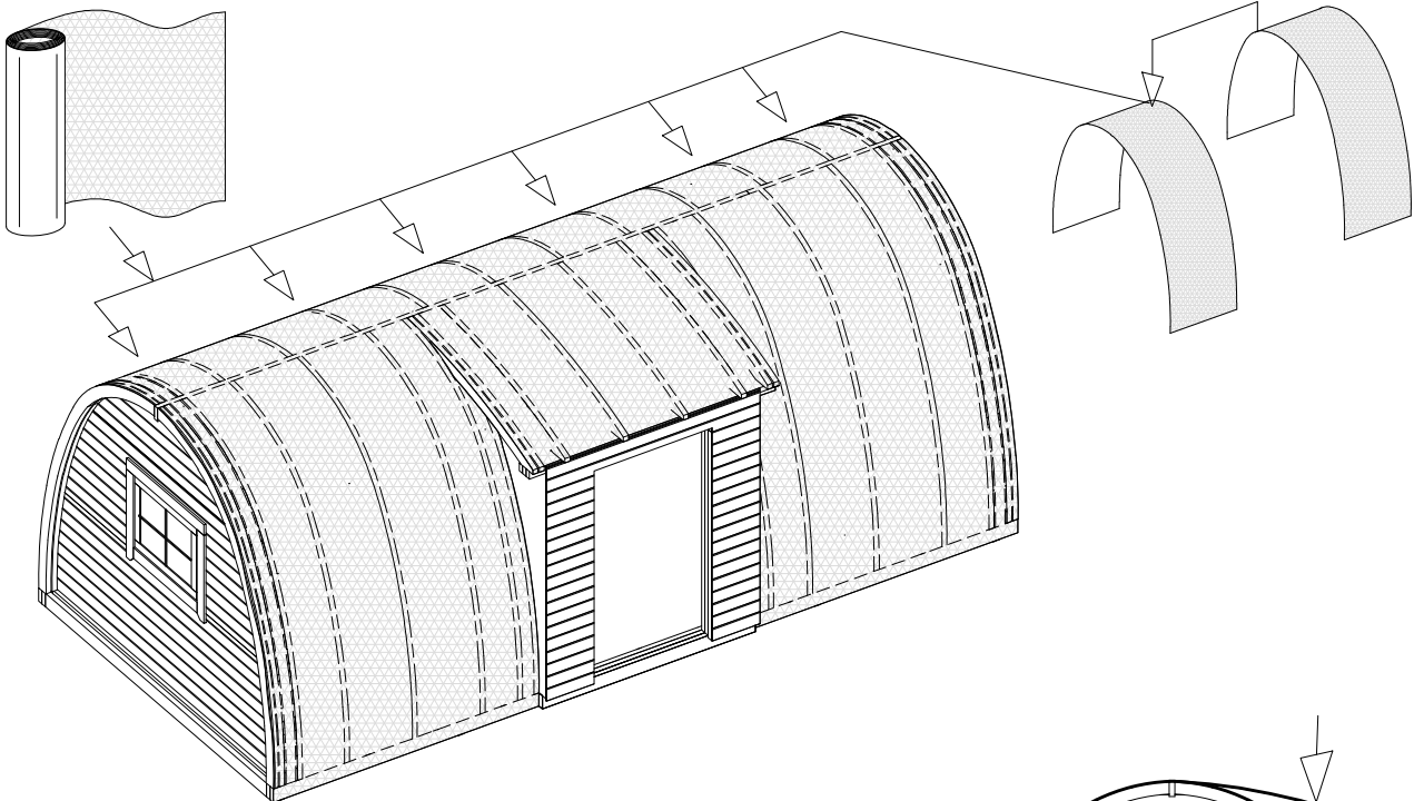
Breather membrane
