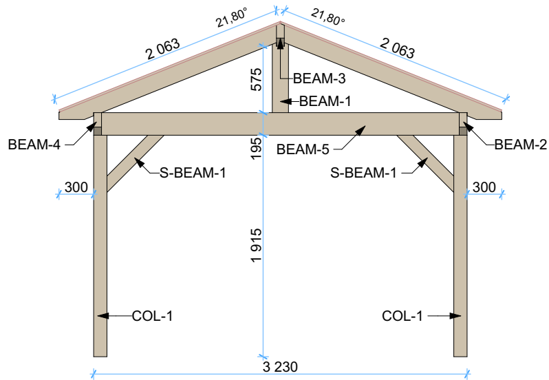
Back Elevation
