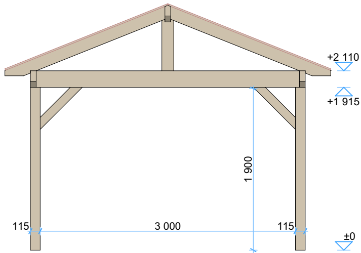
Back Elevation
