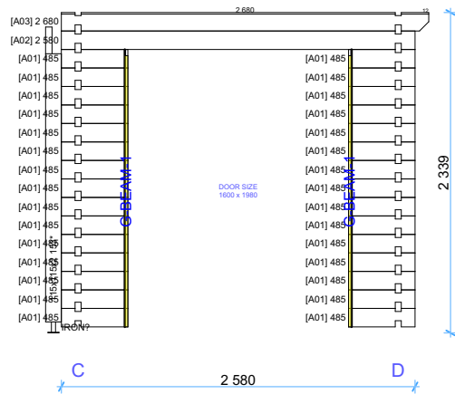
Wall B
