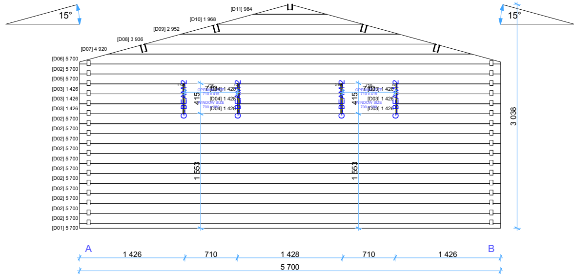
Wall D
