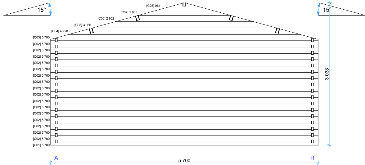
Wall D
