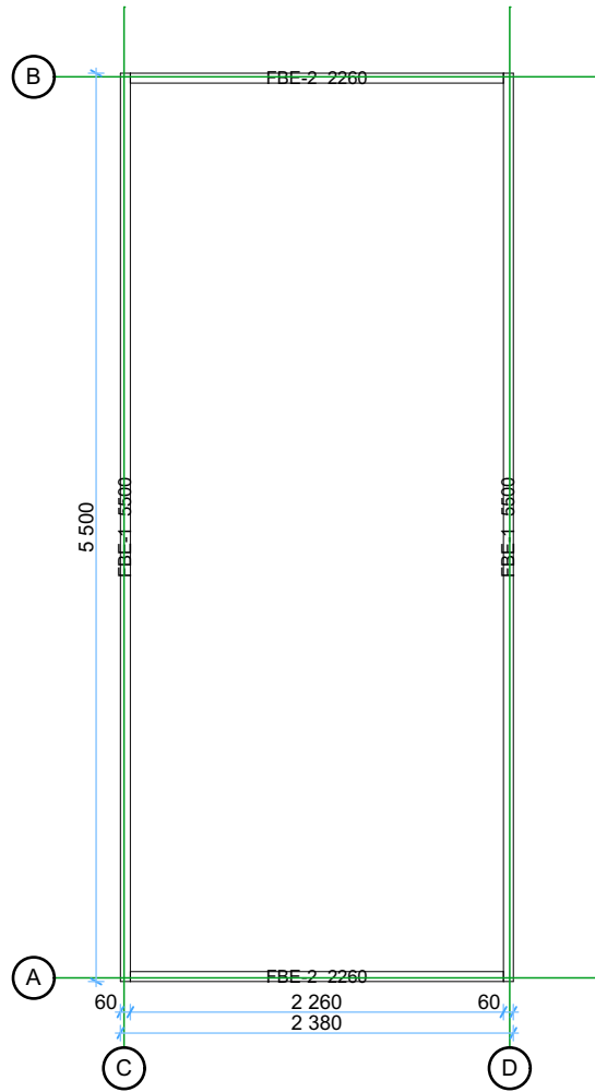
Floor bearers
